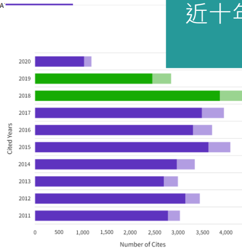
Cited Half-life Data
